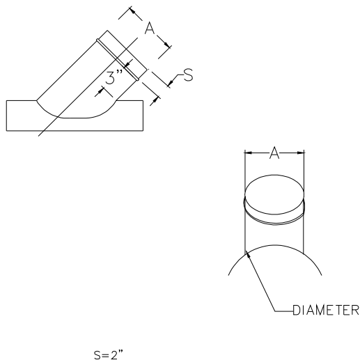
SAD45 SADDLE TAP 45°
