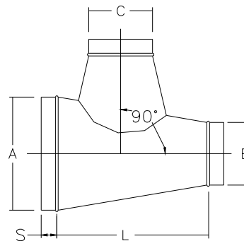
RT90C REDUCING BODY TEE, CONICAL
