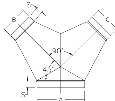
Y45R REDUCING Y-BRANCH 45°
