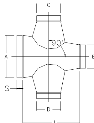
RT90CX REDUCING BODY TEE, CONICAL, CROSS
