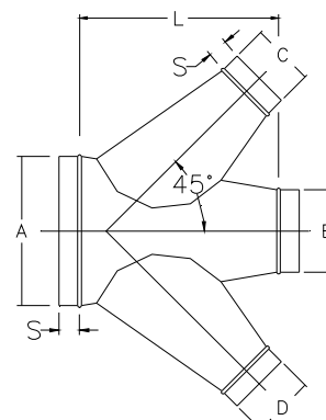
RT45CX REDUCING BODY TEE, LATERAL, CONICAL, CROSS
