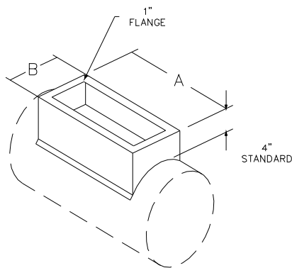
REGB REGISTER BOX
