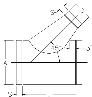
T45C TEE, CONICAL LATERAL
