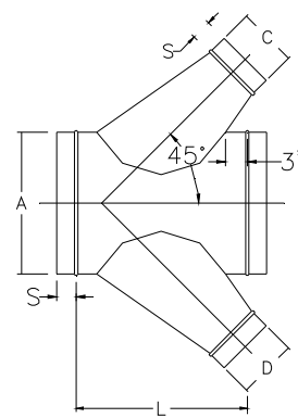
T45XC TEE, CONICAL LATERAL CROSS
