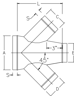
RT45X REDUCING BODY TEE, LATERAL, CROSS
