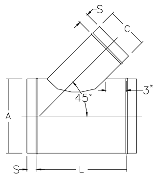
T45 TEE, LATERAL
