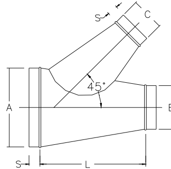
RT45C REDUCING BODY TEE, LATERAL, CONICAL
