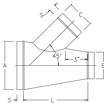
RT45 REDUCING BODY TEE, LATERAL
