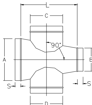
RT90X REDUCING BODY TEE, CROSS
