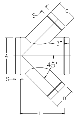
T45X TEE, LATERAL CROSS
