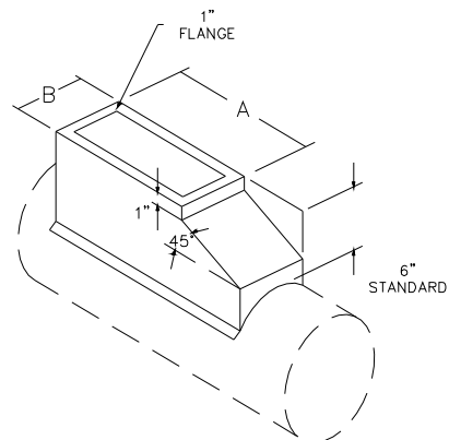
REGB45 REGISTER BOX 45°
