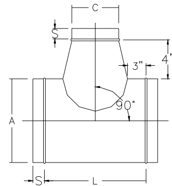
T90C CONICAL TEE
