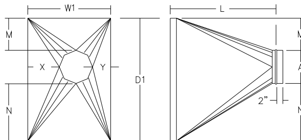
RECTANGULAR TO ROUND NONCONCENTRIC TRANSITION
