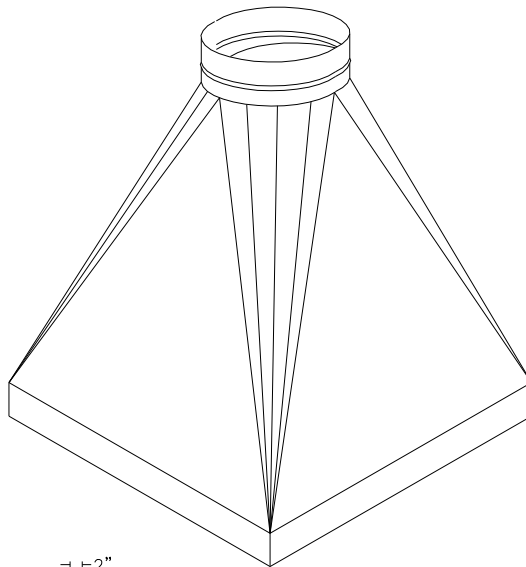
SQRND SQUARE TO ROUND TRANSITIONS
