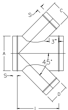
T45X TEE, LATERAL CROSS
