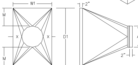
RECTANGULAR TO ROUND CONCENTRIC TRANSITION
